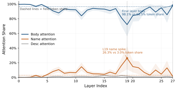
(a) Attention Deviates From Length Baselines
