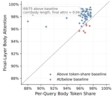
(b) Query-Level Final-Layer Check
