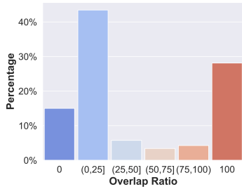
GrailQA
