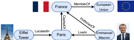
Knowledge Graphs
