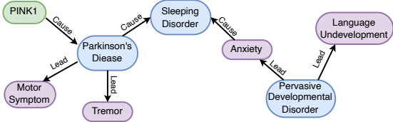
Knowledge Graph
