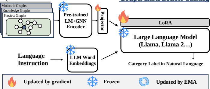
Figure 1: Overview of UniGraph framework. 1) In pre-training, we employ a self-supervised approach, leveraging TAGs to unify diverse graph data. This phase involves a cascaded architecture combining LMs and GNNs. We propose Graph Siamese
