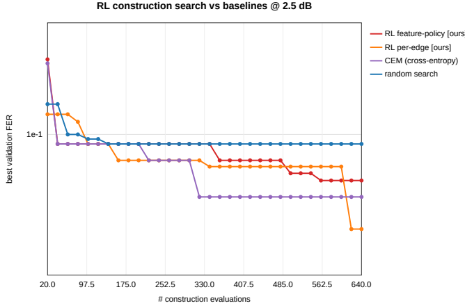
Fig. 2. Best validation FER vs. number of construction evaluations. Random search stalls at \approx 0.09 ; RL (both policies) and CEM keep descending via a structured policy.
