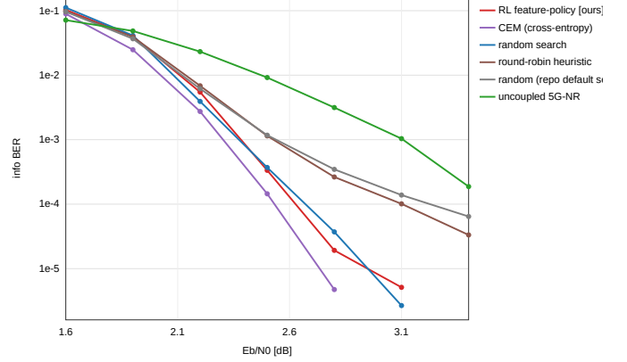
Fig. 1. BER-vs- E_b/N_0 waterfall for six constructions. Optimized constructions (RL/CEM/random search) decay without a floor; the repository default (seed-0) and the naive round-robin heuristic exhibit an error floor at \approx 3\text{--}6 \times 10^{-5} ; the uncoupled component code is worst.
