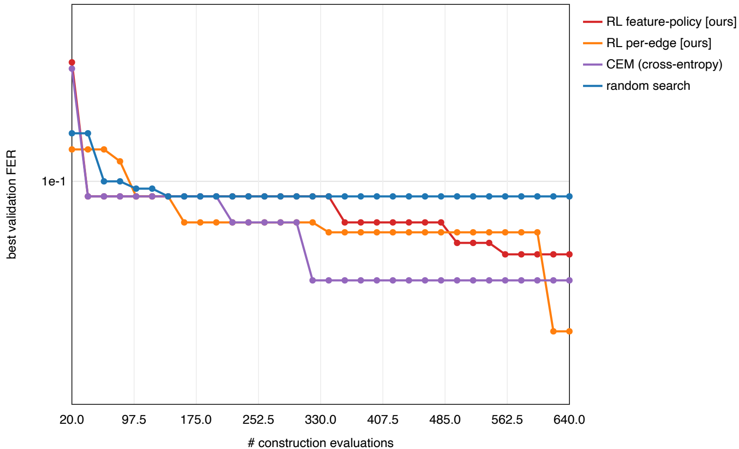
RL construction search vs baselines @ 2.5 dB
