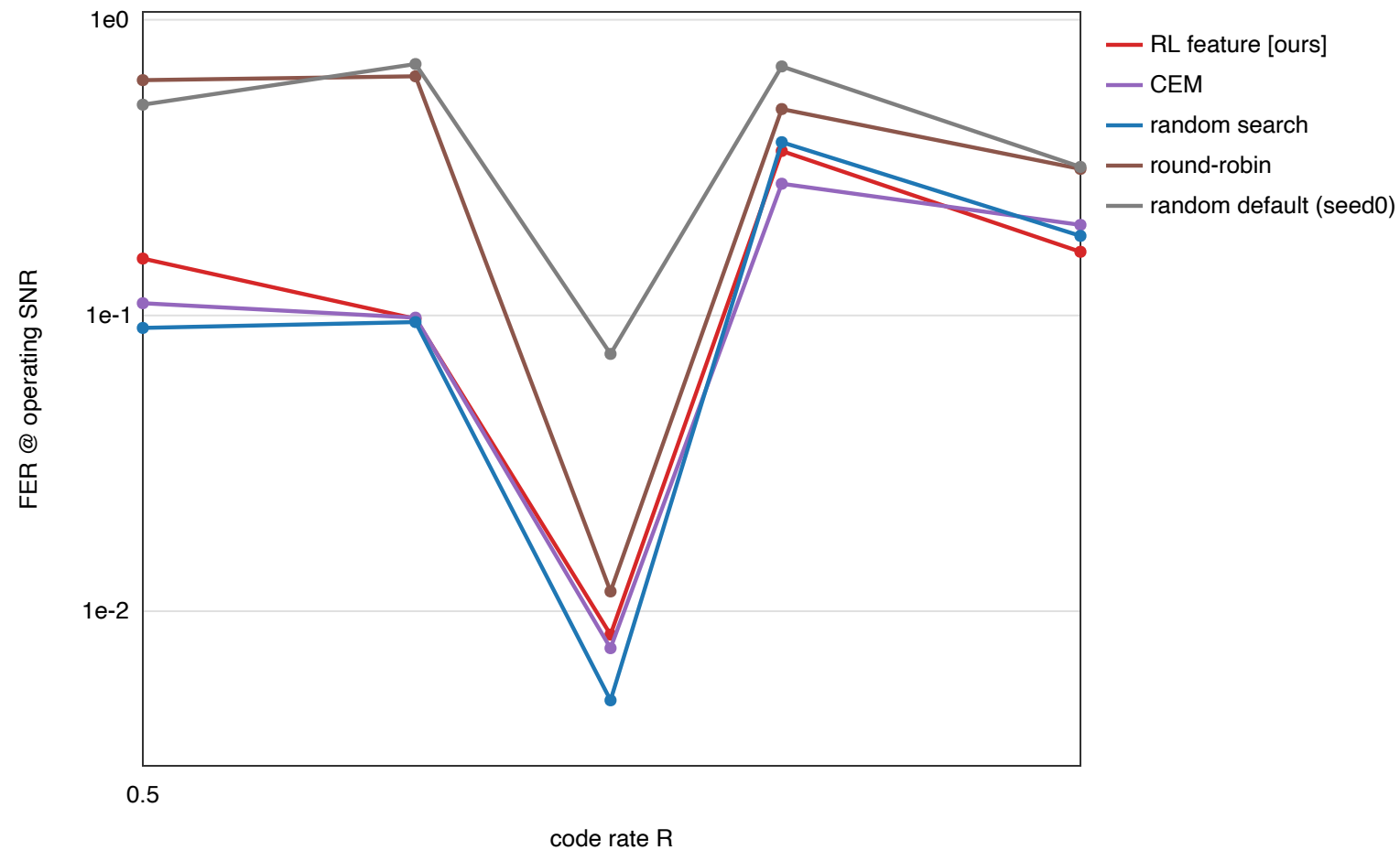
RL-optimized SC-LDPC construction across rates 0.5-0.9
