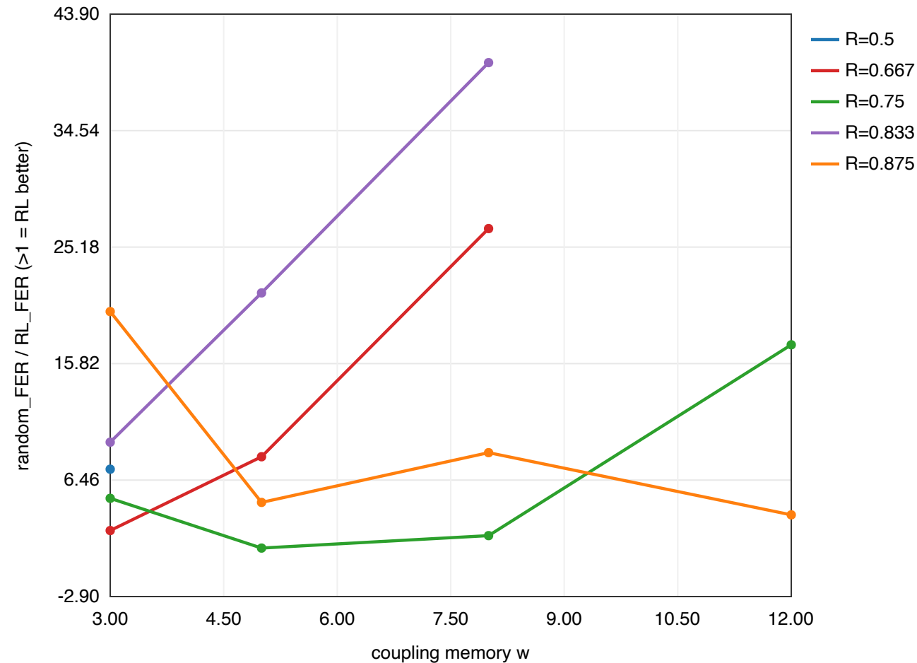
RL vs random search vs w (Monte-Carlo, long Z=32 codes)
