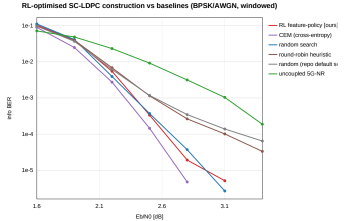
Fig. 3. BER-vs- E_b/N_0 waterfall for six constructions. Optimized constructions (RL/CEM/random search) decay without a floor; the repository default (seed-0) and the naive round-robin heuristic exhibit an error floor at \approx 3\text{--}6 \times 10^{-5} ; the uncoupled component code is worst.
