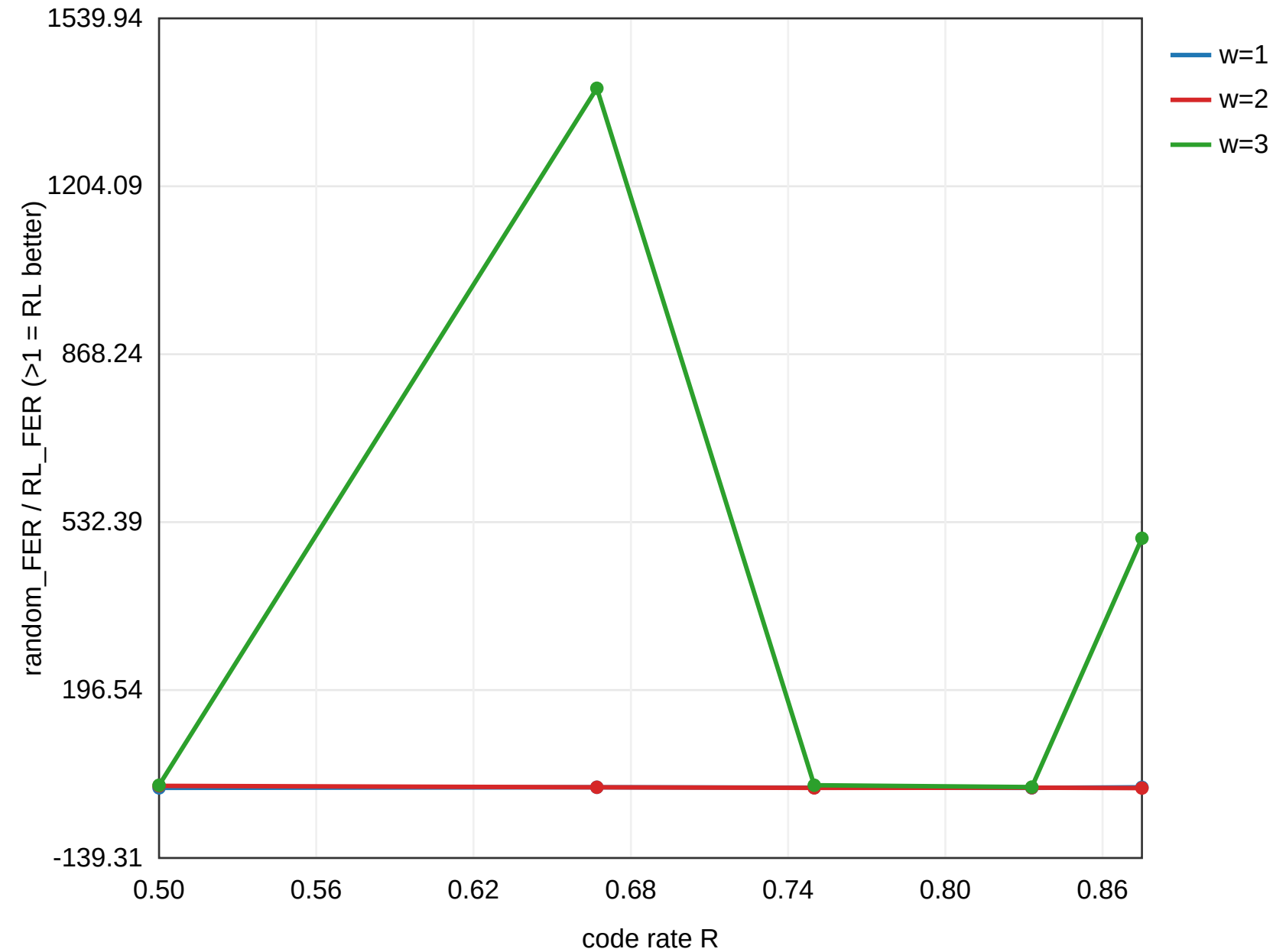
RL vs equal-budget random search across rate x w (long Z=64 codes)
