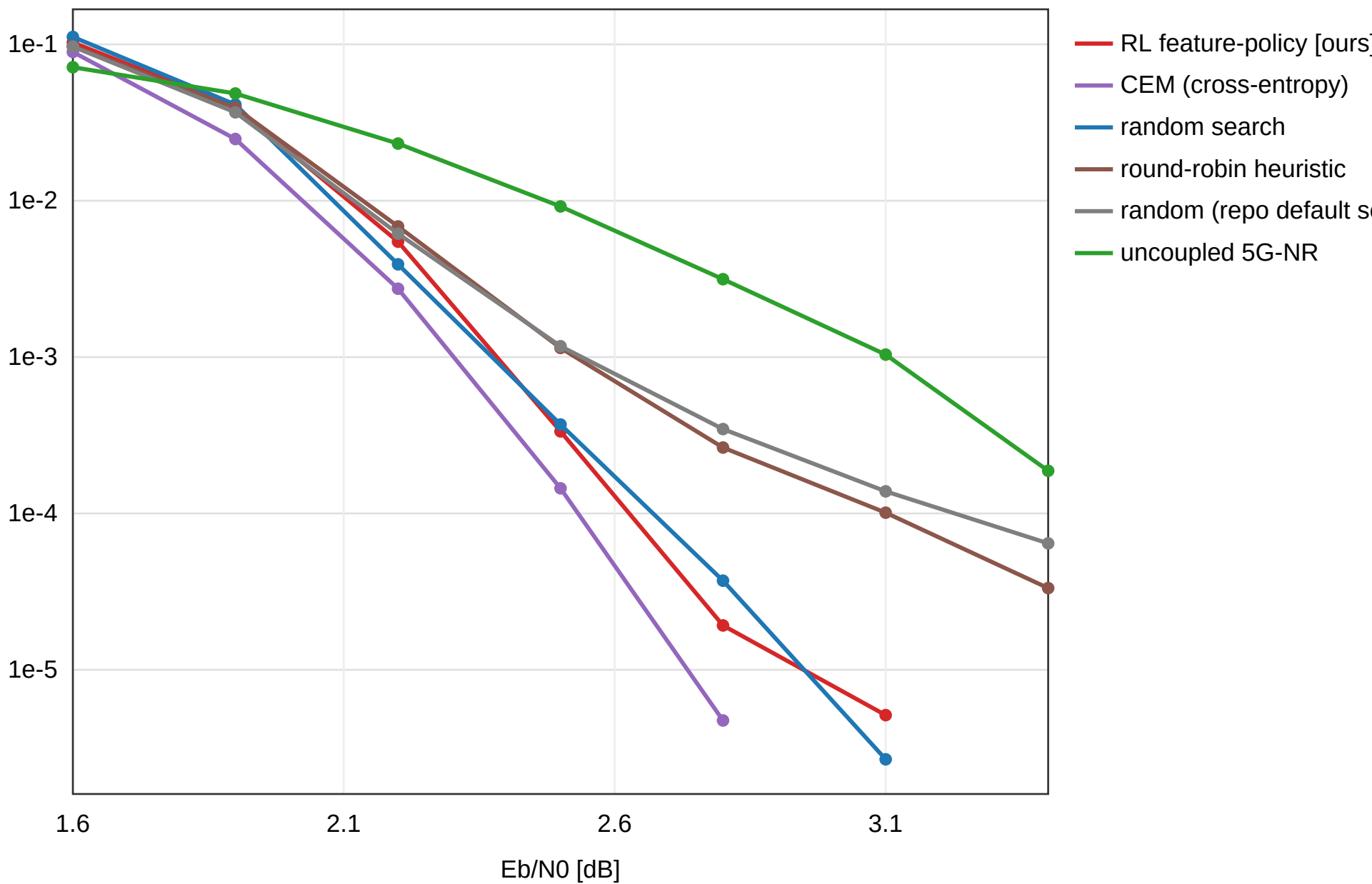
RL-optimised SC-LDPC construction vs baselines (BPSK/AWGN, windowed)
