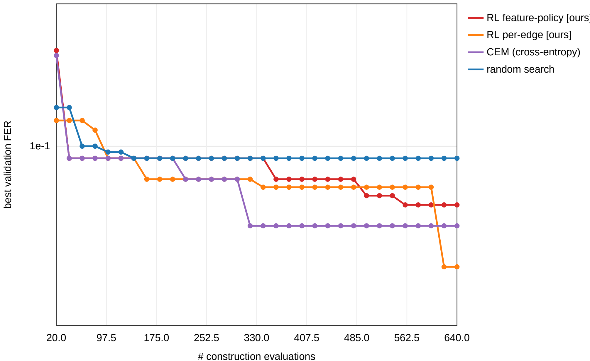
RL construction search vs baselines @ 2.5 dB
