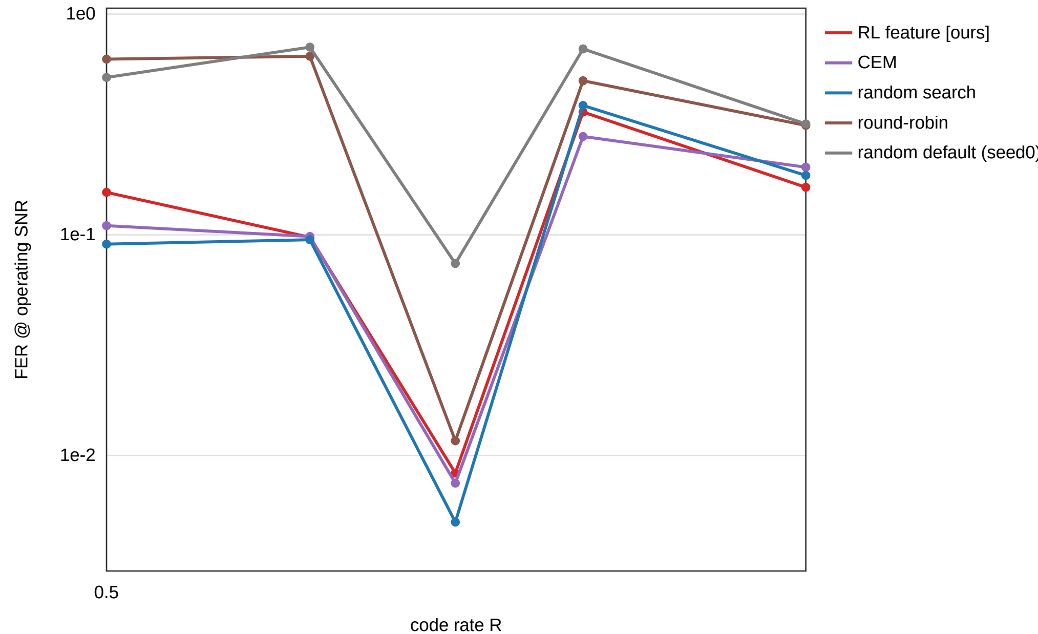
RL-optimized SC-LDPC construction across rates 0.5-0.9
