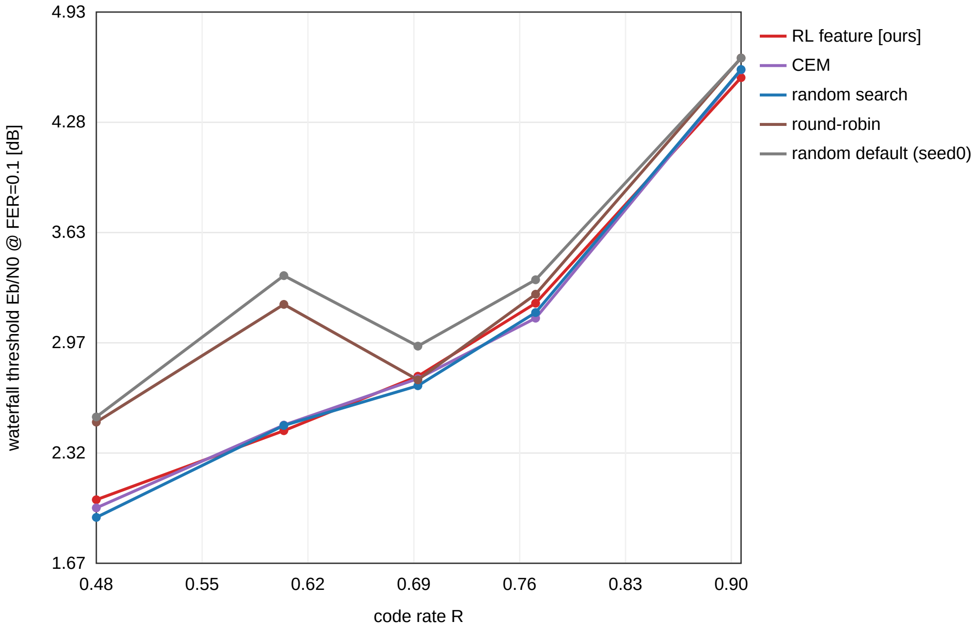
RL-optimized SC-LDPC construction across rates (lower=better)
