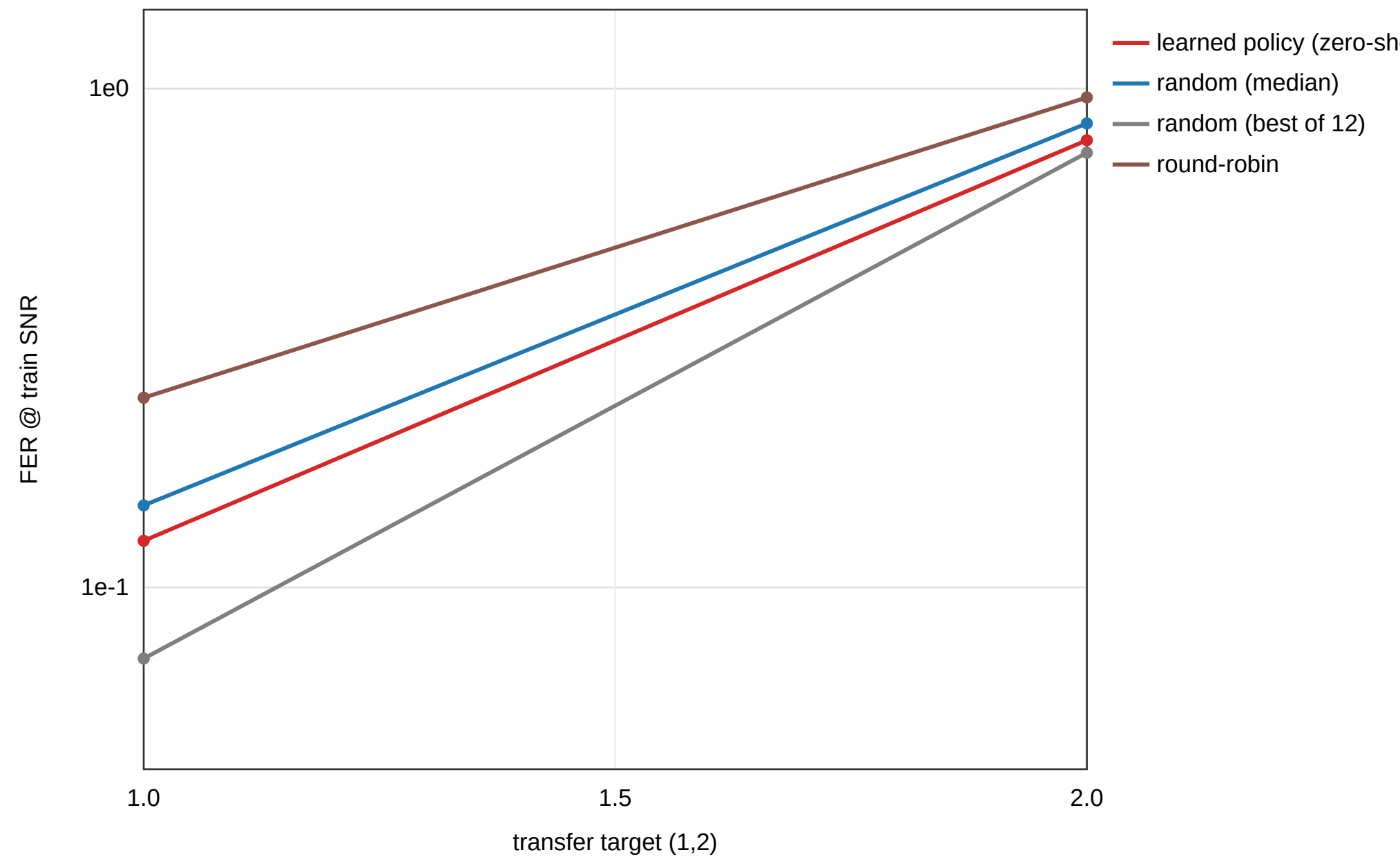
Zero-shot transfer of the learned construction policy
