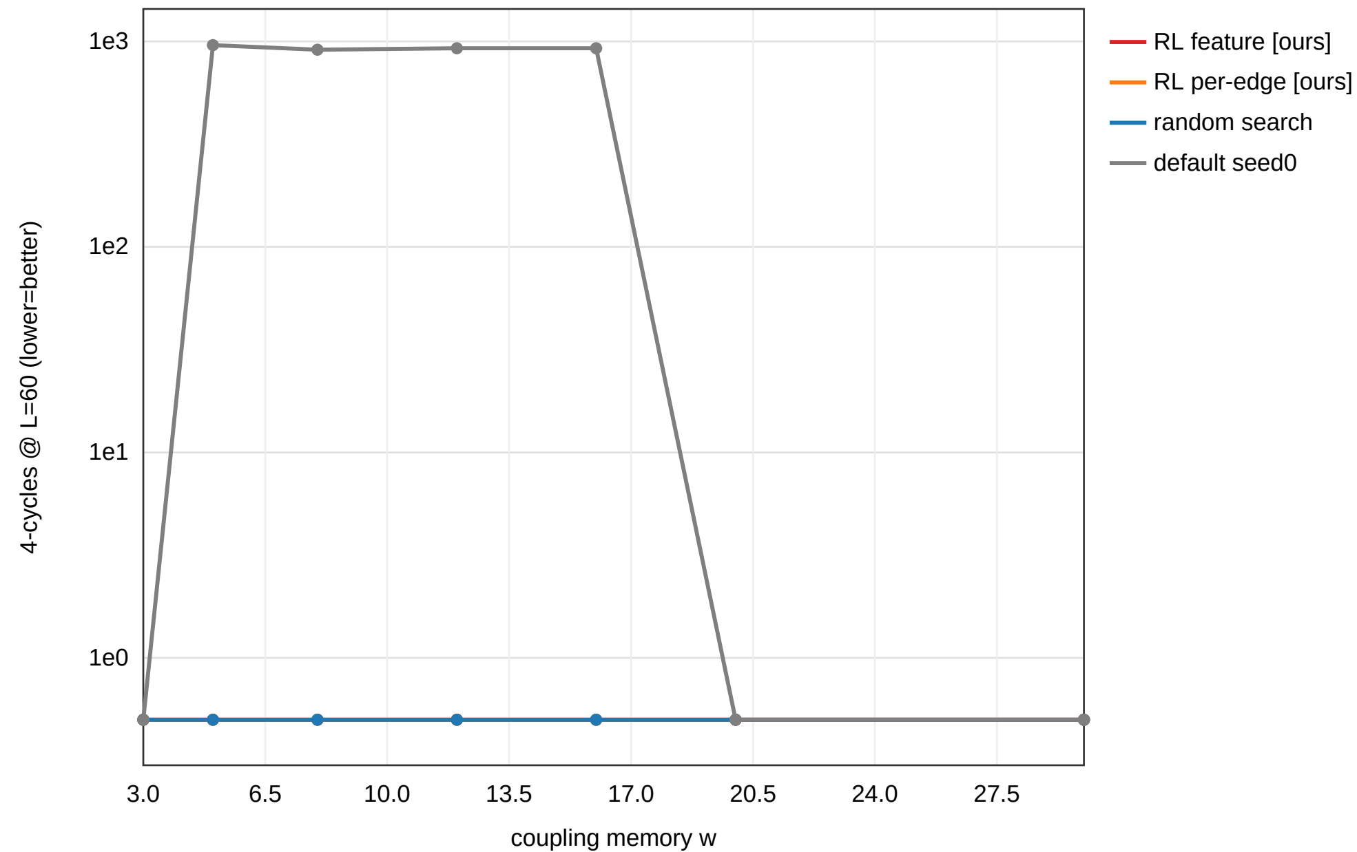
RL minimises coupled-graph 4-cycles across w (BG1 Z=16, R~2/3)
