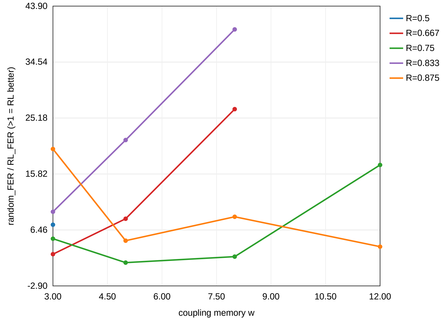
RL vs random search vs w (Monte-Carlo, long Z=32 codes)
