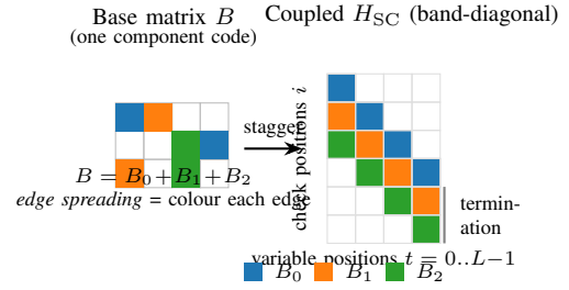
Fig. 1. Edge spreading and the resulting spatially-coupled code. (a) A single base protograph B is split into w+1 components by assigning each base edge to one of B_0, B_1, B_2 (a colouring). (b) Staggering the components along the diagonal yields the band-diagonal coupled matrix H_{SC}[i, t] = B_{i-t} over coupling length L ; the last w check positions are the termination. The colouring in (a)—i.e. which edge goes to which component—is the construction variable this paper optimizes; in standard pipelines it is drawn from a random number generator.
