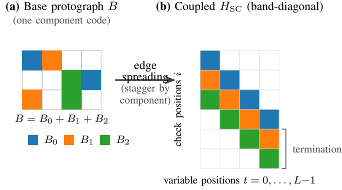
Fig. 1. Edge spreading and the resulting spatially-coupled code. (a) A single base protograph B is split into w+1 components by assigning each base edge to one of B_0, B_1, B_2 (a colouring). (b) Staggering the components along the diagonal yields the band-diagonal coupled matrix H_{SC}[i, t] = B_{i-t} over coupling length L ; the last w check positions are the termination. The colouring in (a)—which edge goes to which component—is the construction variable this paper optimizes; in standard pipelines it is drawn from a random number generator.
