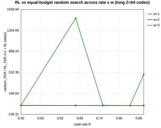
Fig. 6. RL-vs-random-search advantage across the long-code cells, by rate and coupling memory w . The advantage is systematic and grows with w (search-space size).
