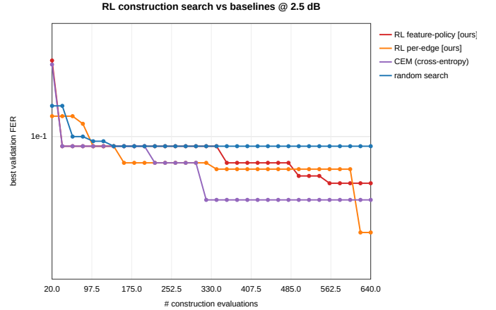
Fig. 2. Best validation FER vs. number of construction evaluations (single representative seed; cf. Table III for across-seed CIs). Random search stalls early; RL (both policies) and CEM keep descending via a structured policy.
