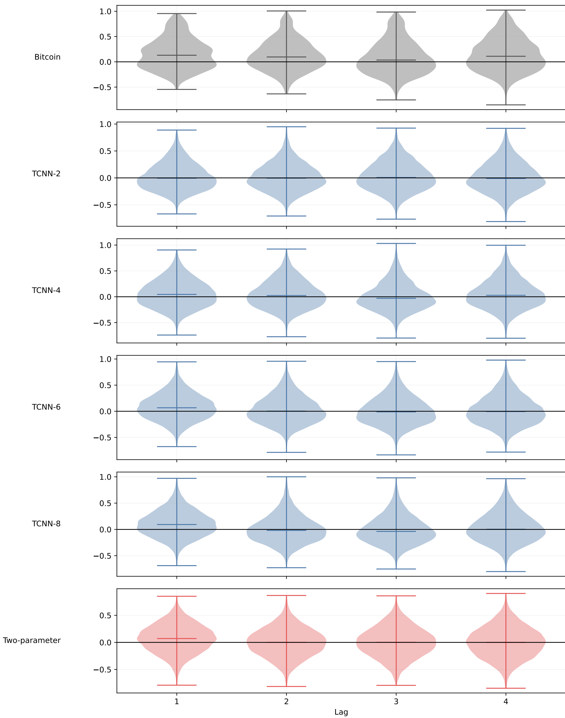
Window-level absolute-return ACF distributions
