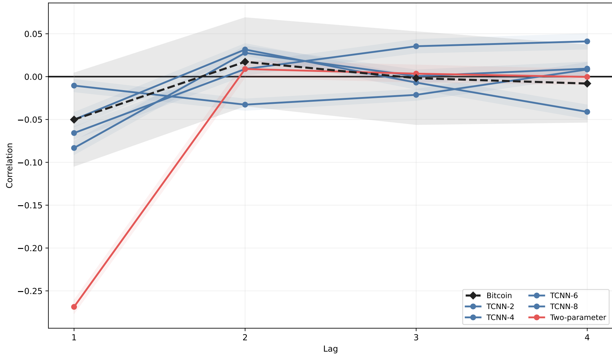
Classical WGAN: Raw-return ACF
