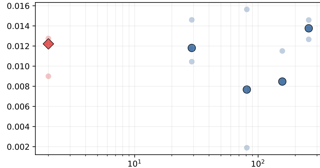
Leverage MAE, lags 1-4
