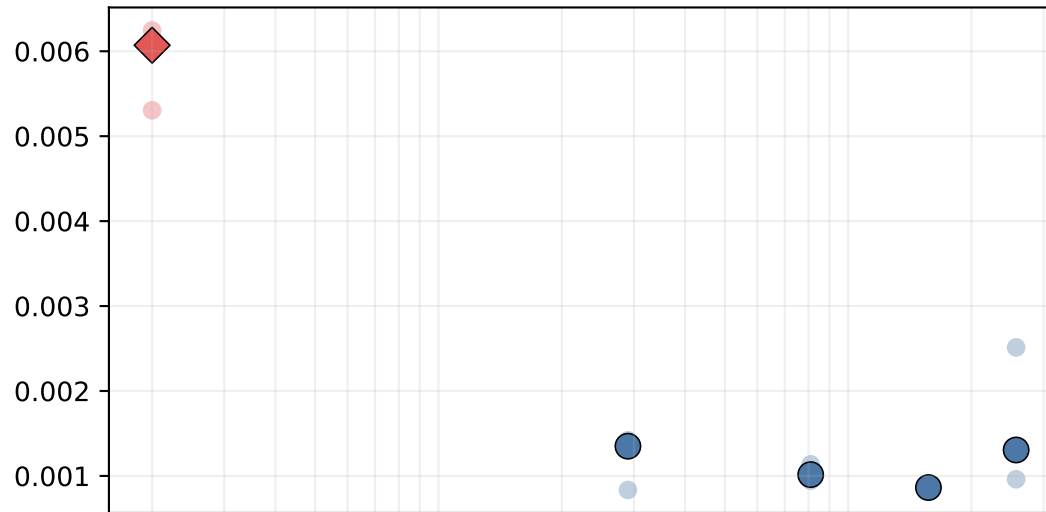
Fresh-sample marginal Wasserstein distance
