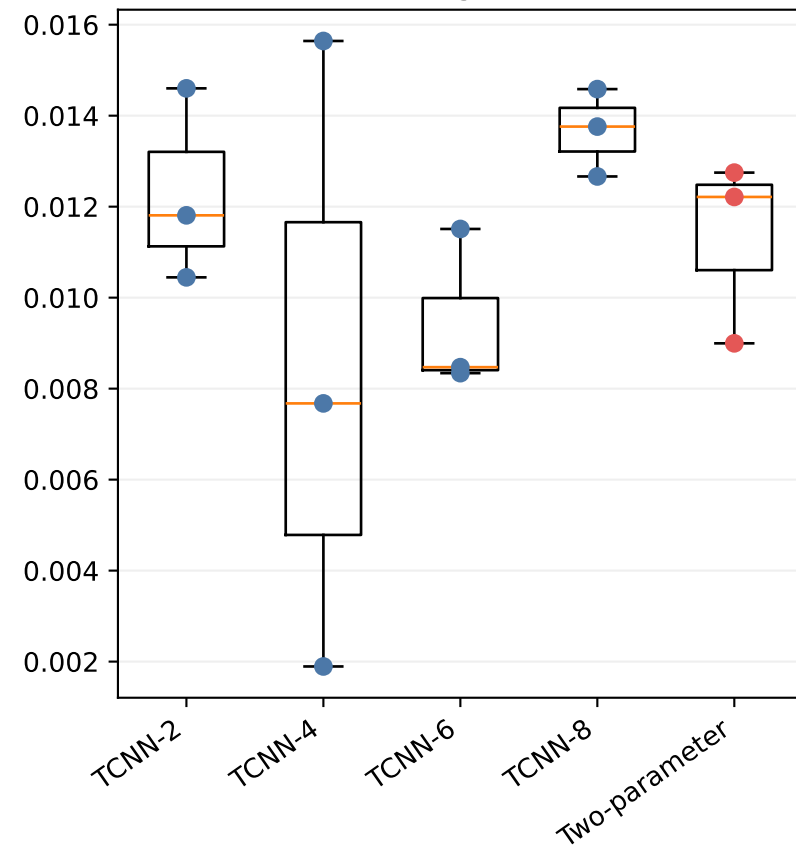
Leverage MAE
