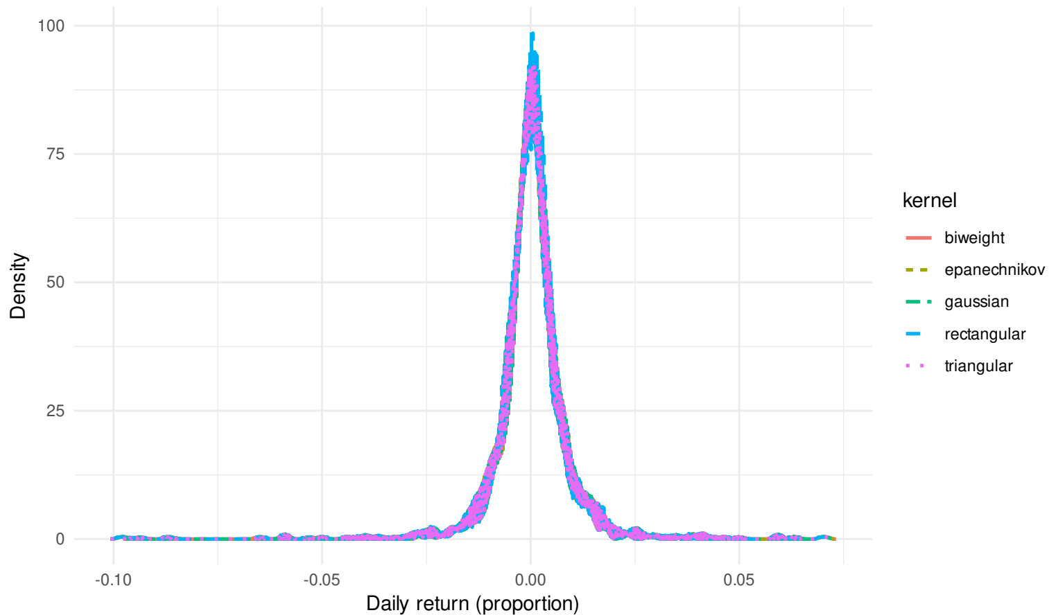
Overlay kernels (avg over weekdays) | fd | bw: bw_nrd0
