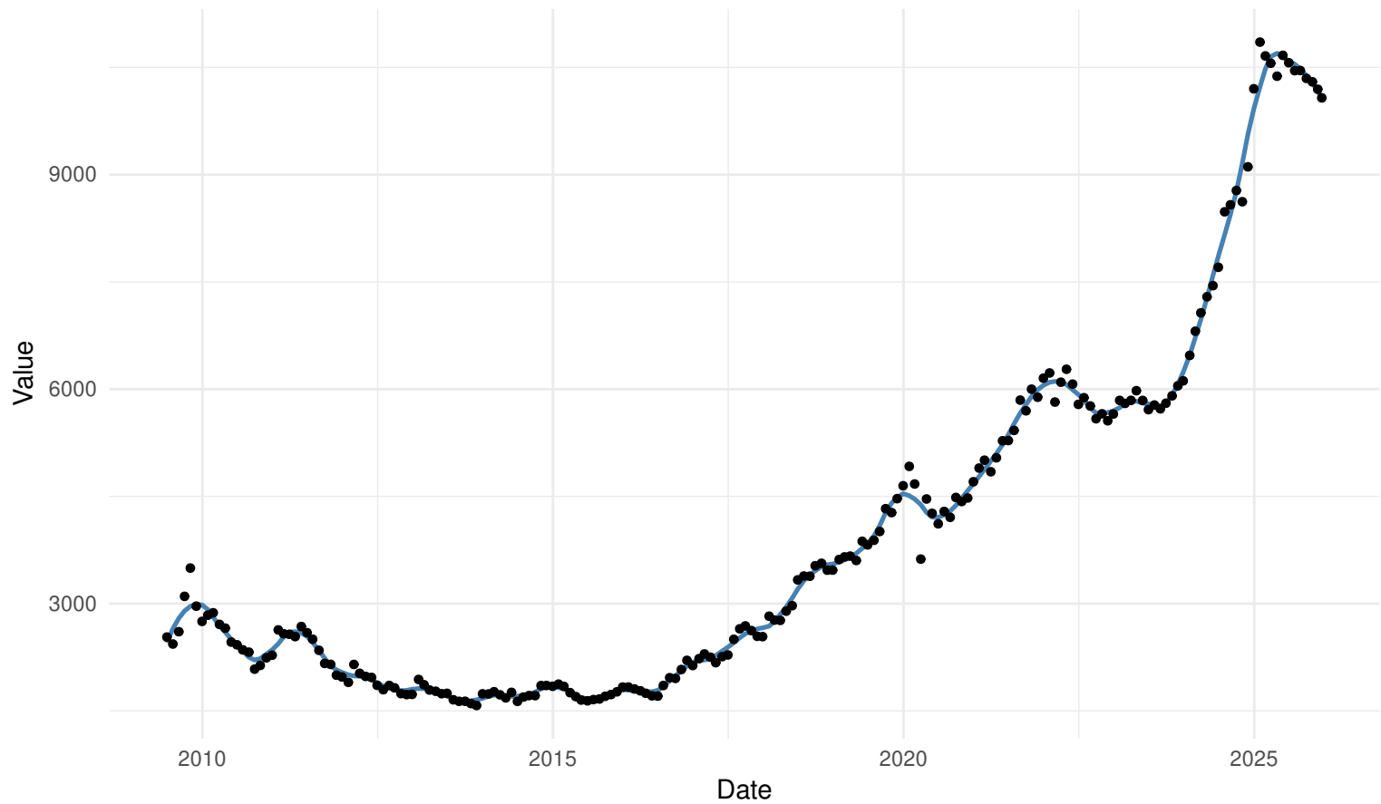
MONTHLY local regression: kernel=biweight | bw=SJ
