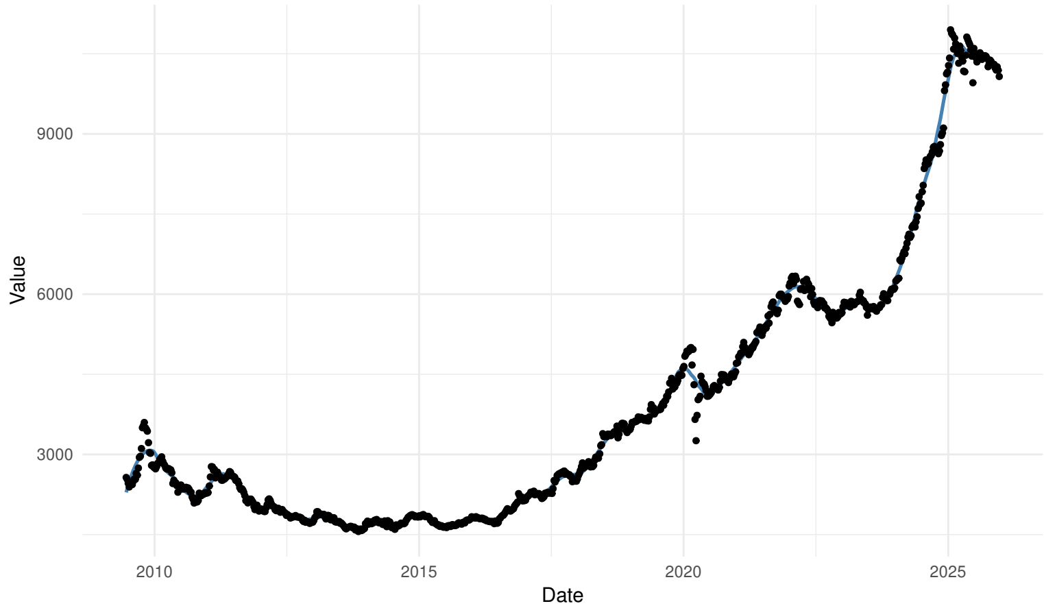
WEEKLY local regression: kernel=gaussian | bw=nrd0
