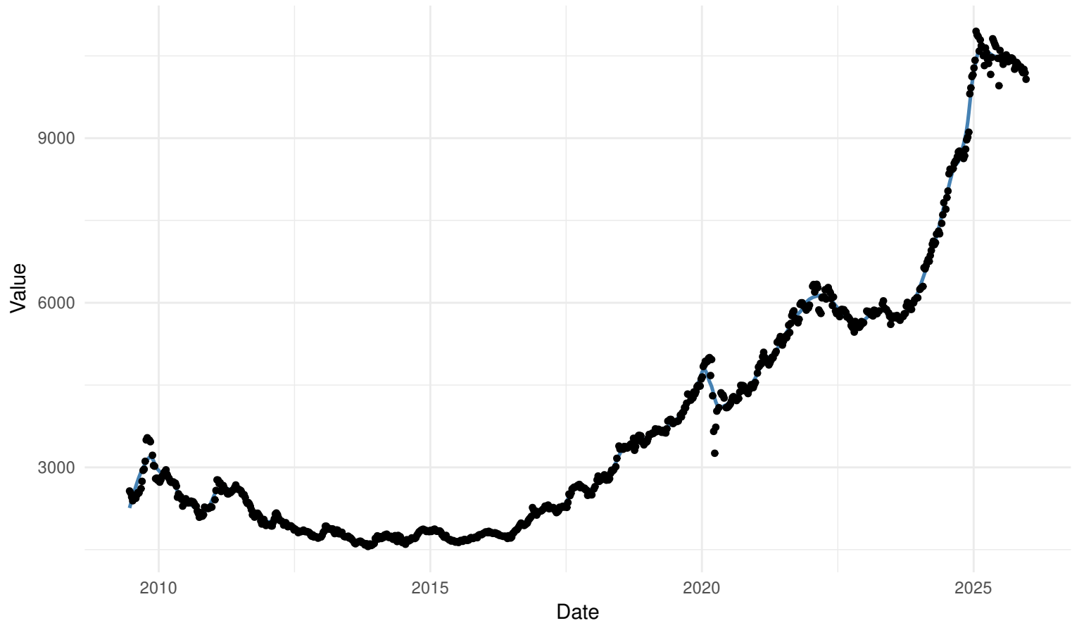
WORKDAYS Friday local regression: kernel=biweight | bw=ucv
