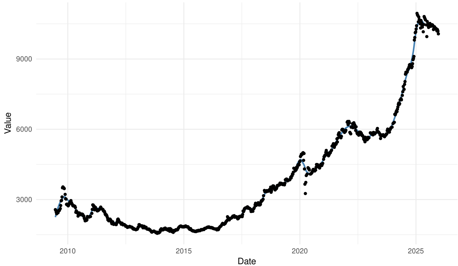
WORKDAYS Friday local regression: kernel=epanechnikov | bw=SJ
