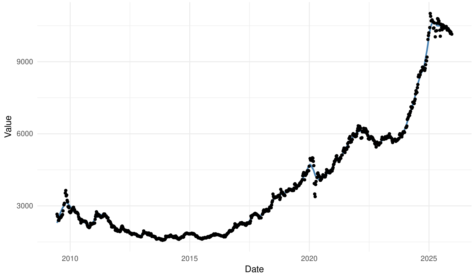
WORKDAYS Monday local regression: kernel=triangular | bw=SJ
