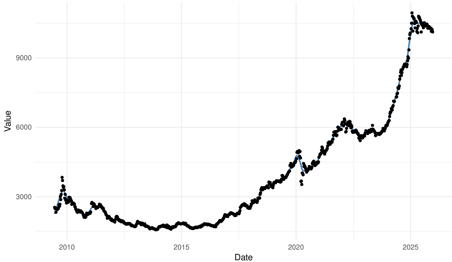
WORKDAYS Wednesday local regression: kernel=epanechnikov | bw=ucv
