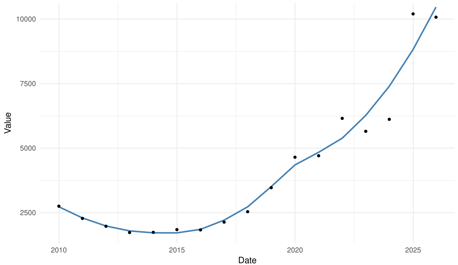
YEARLY local regression: kernel=rectangular | bw=nrd0
