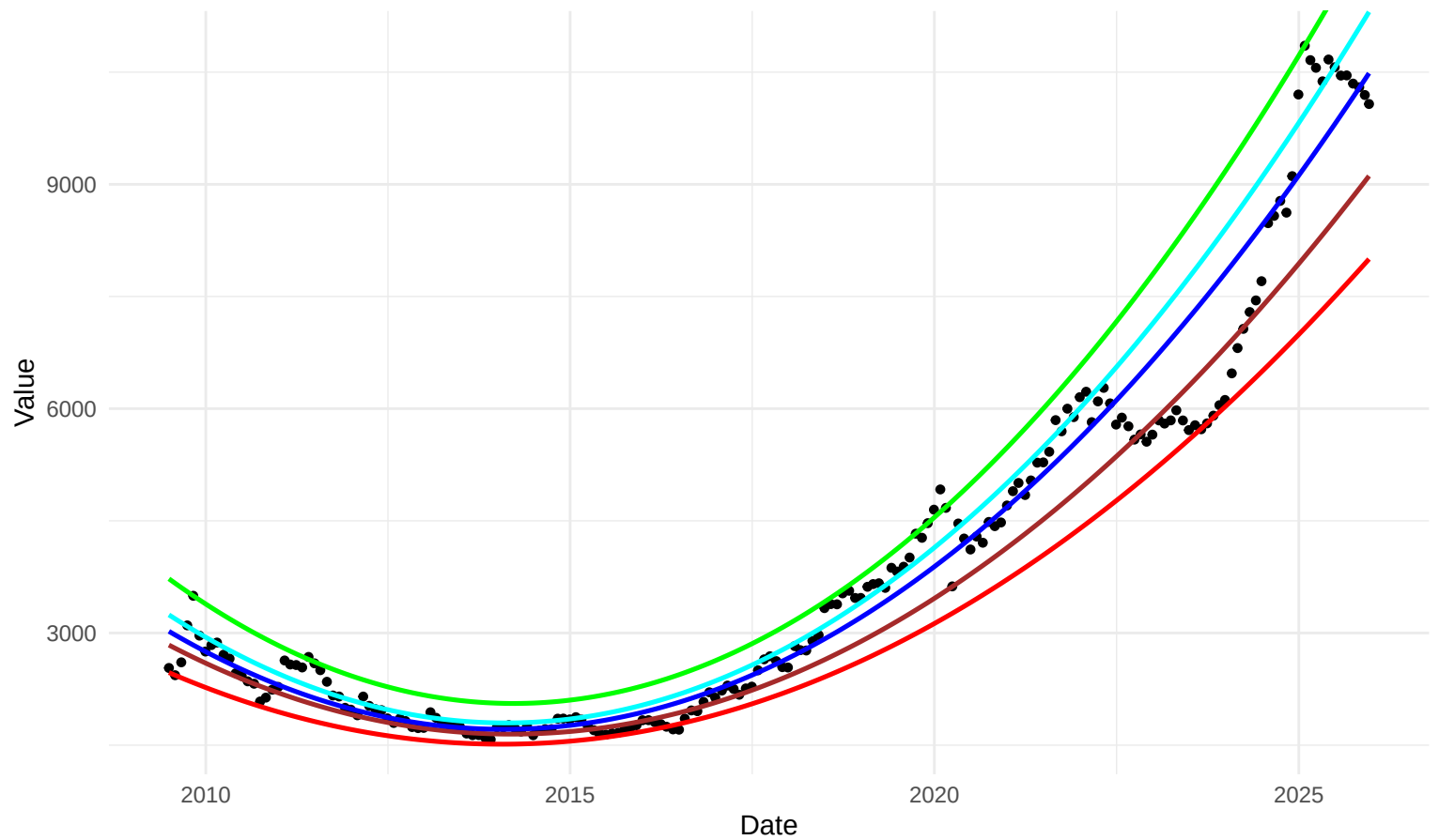
MONTHLY Quantile Regression
