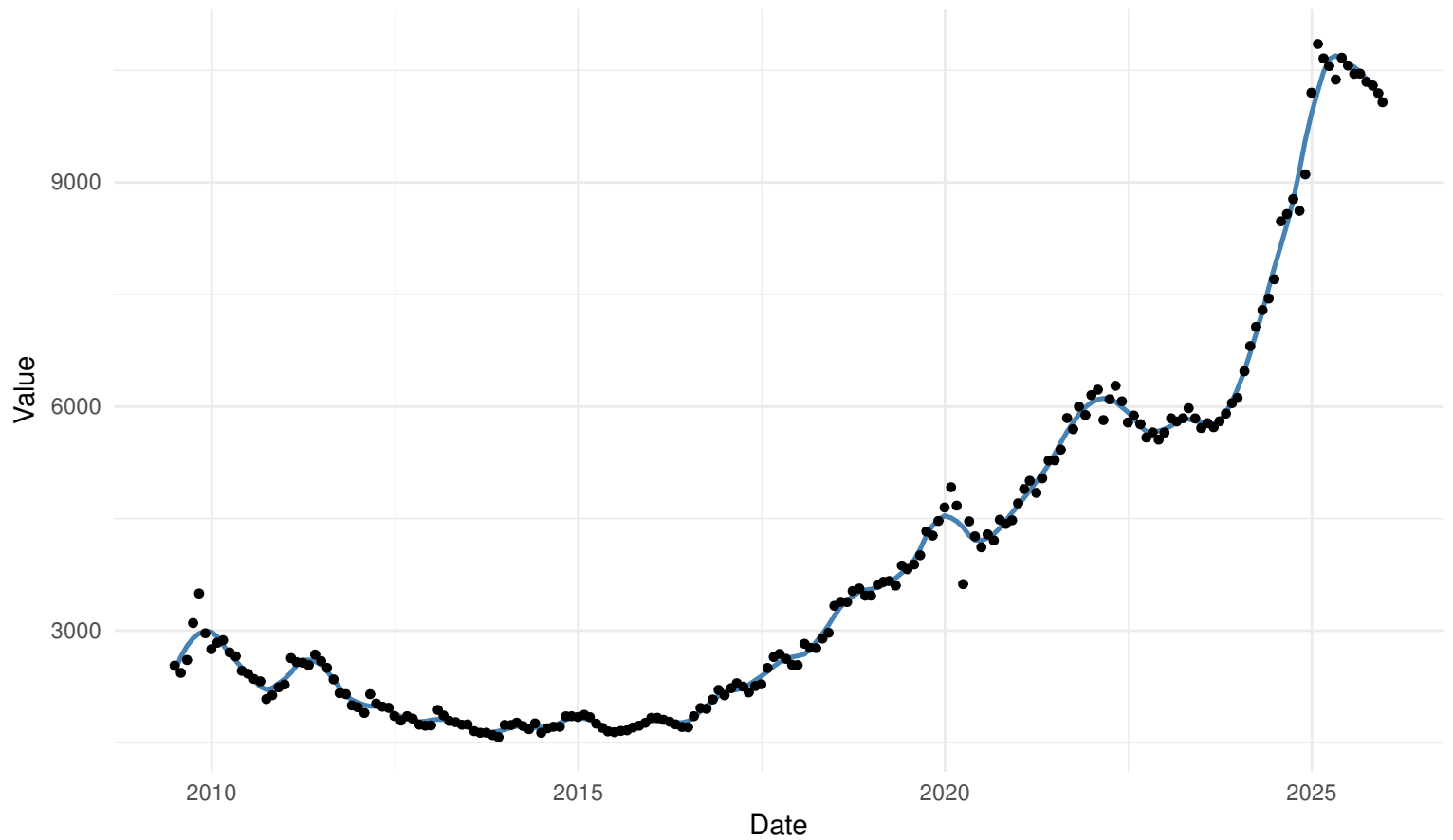
MONTHLY local regression: kernel=epanechnikov | bw=SJ
