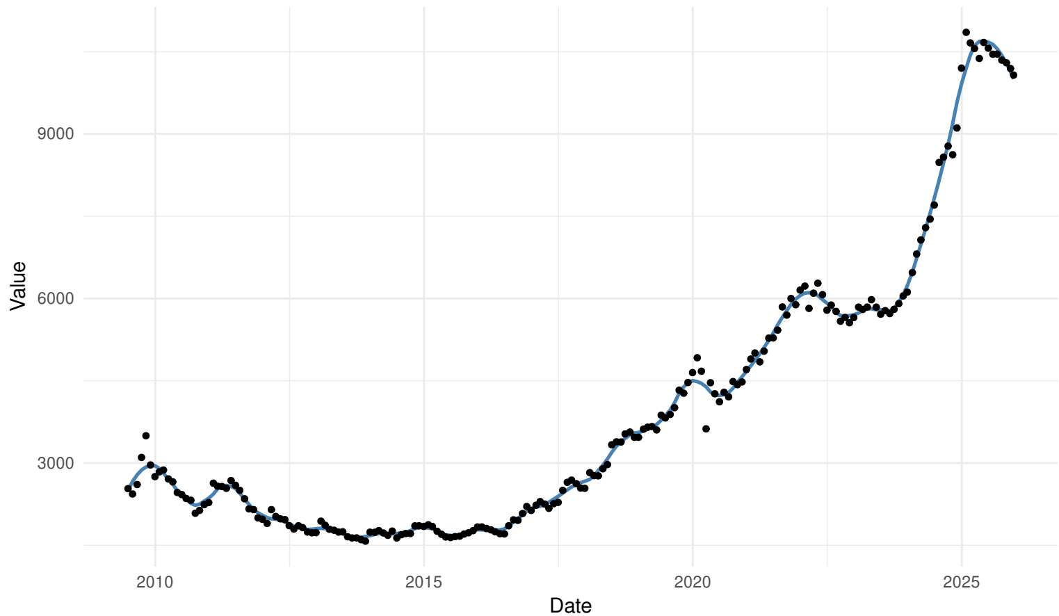
MONTHLY local regression: kernel=rectangular | bw=ucv
