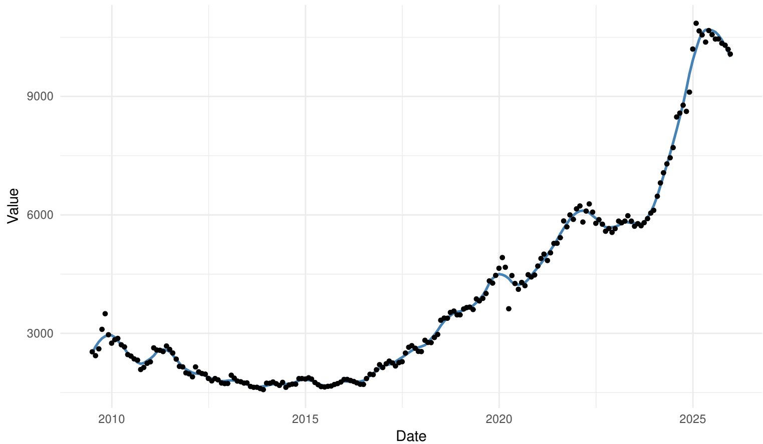
MONTHLY local regression: kernel=triangular | bw=nrd0
