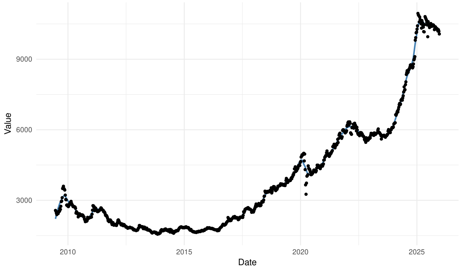
WEEKLY local regression: kernel=rectangular | bw=SJ
