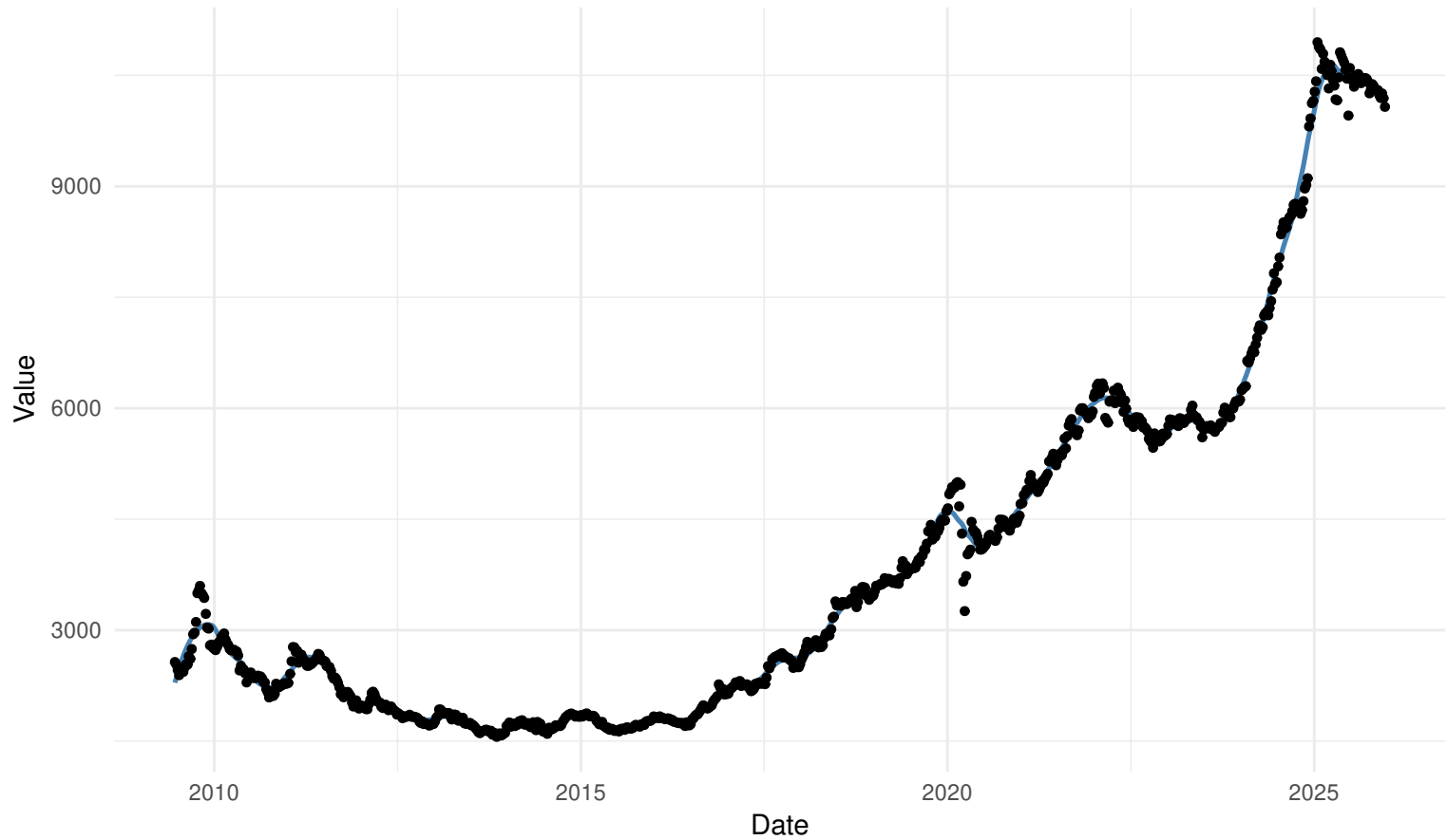
WEEKLY local regression: kernel=triangular | bw=nrd0
