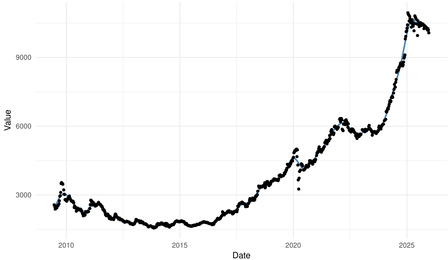
WORKDAYS Friday local regression: kernel=rectangular | bw=nrd0
