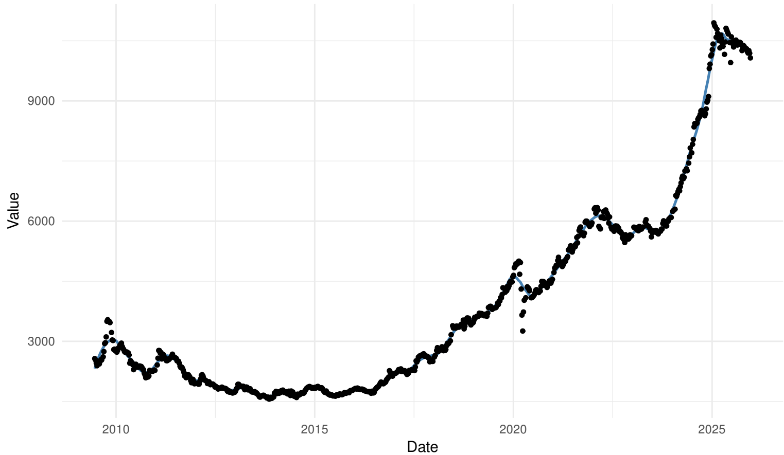
WORKDAYS Friday local regression: kernel=triangular | bw=nrd0
