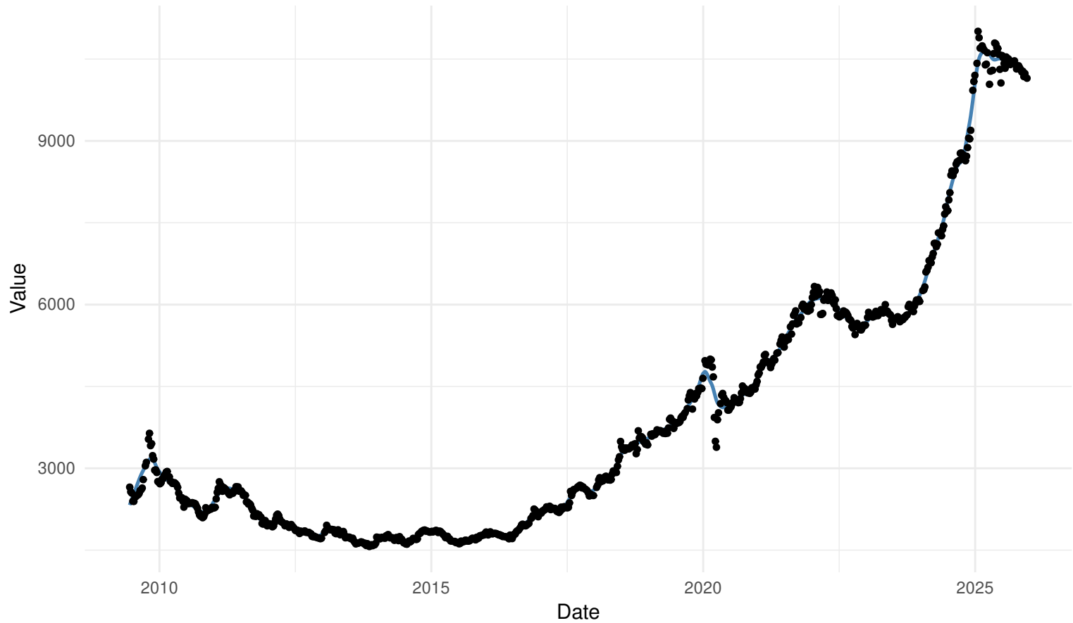
WORKDAYS Monday local regression: kernel=biweight | bw=ucv
