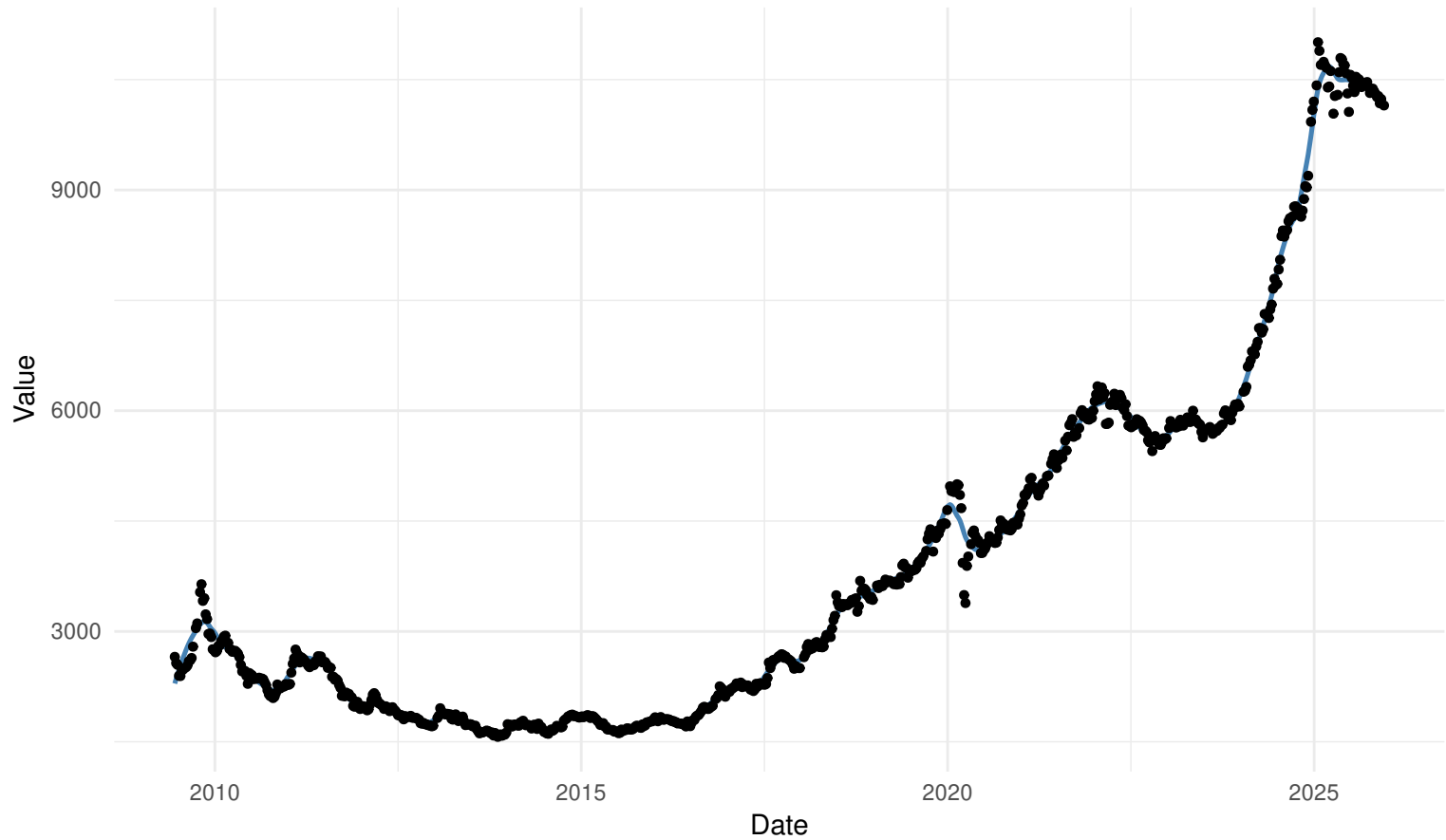
WORKDAYS Monday local regression: kernel=epanechnikov | bw=SJ
