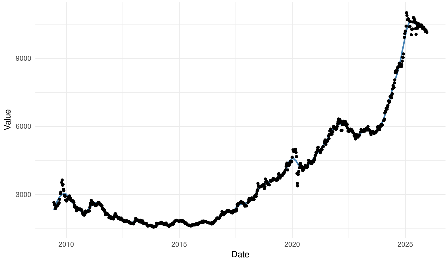
WORKDAYS Monday local regression: kernel=rectangular | bw=nrd0
