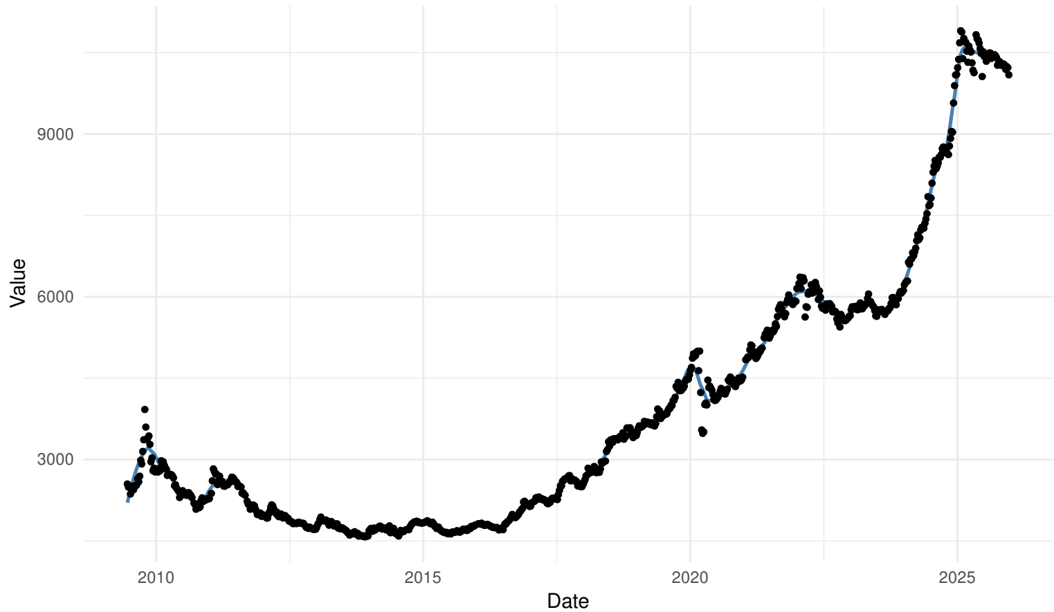
WORKDAYS Thursday local regression: kernel=epanechnikov | bw=SJ
