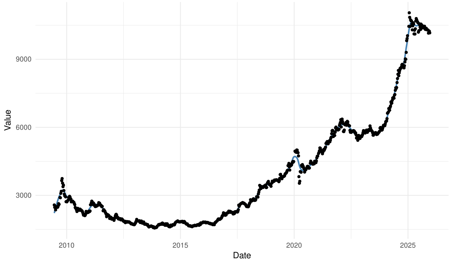
WORKDAYS Tuesday local regression: kernel=triangular | bw=ucv
