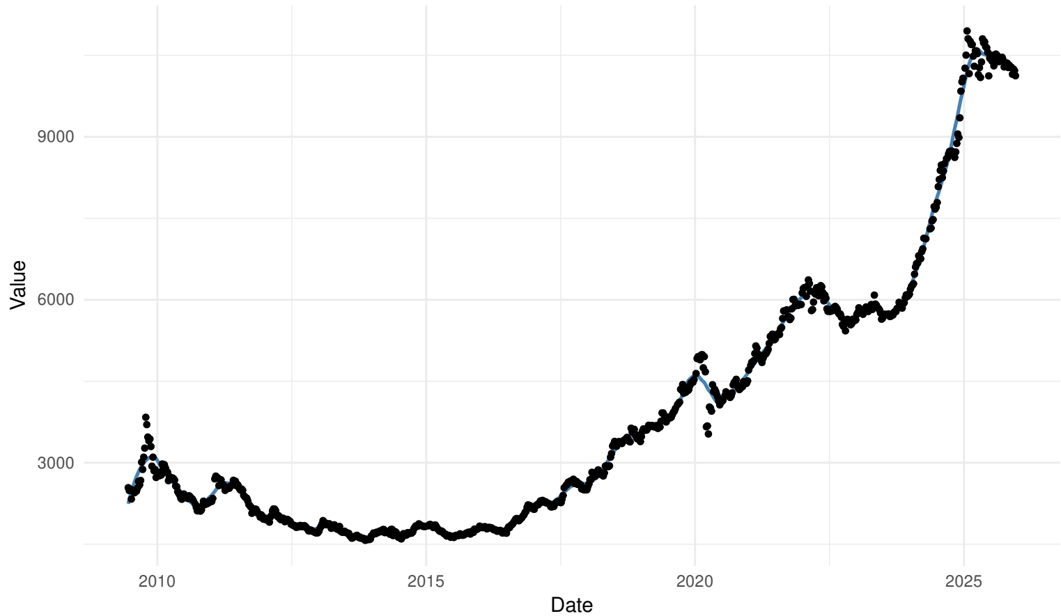
WORKDAYS Wednesday local regression: kernel=biweight | bw=nrd0
