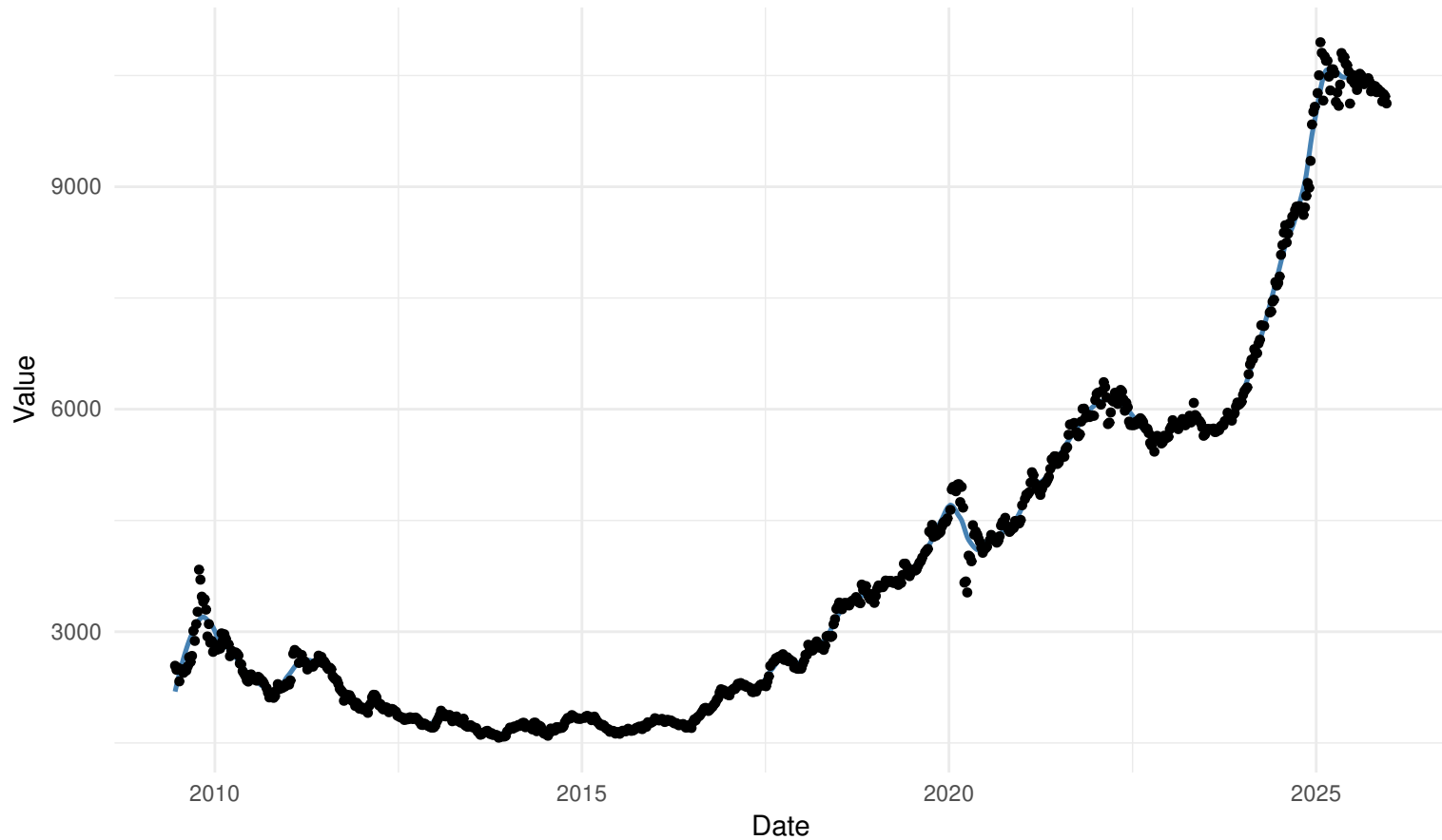
WORKDAYS Wednesday local regression: kernel=gaussian | bw=SJ
