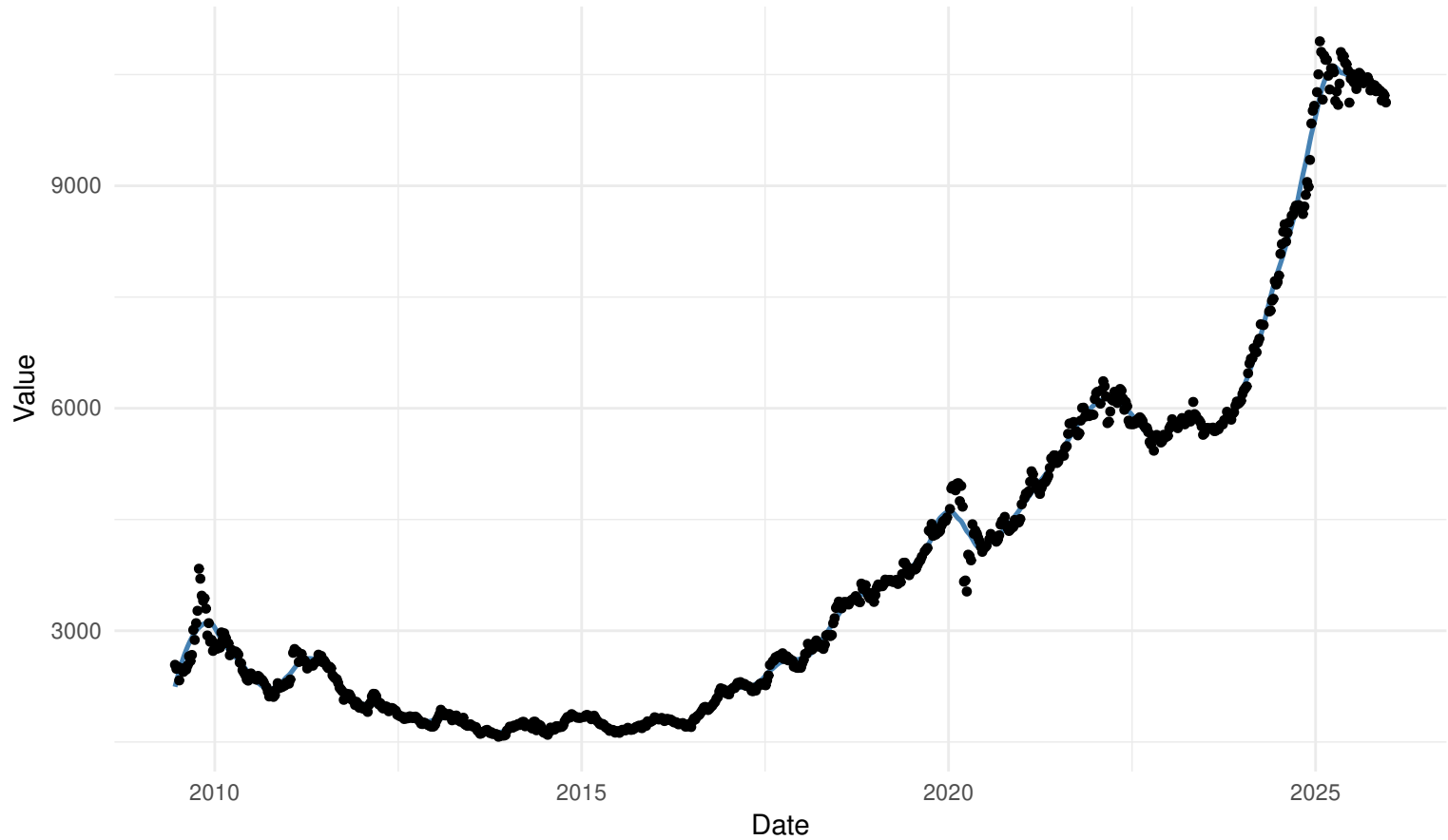
WORKDAYS Wednesday local regression: kernel=rectangular | bw=nrd0
