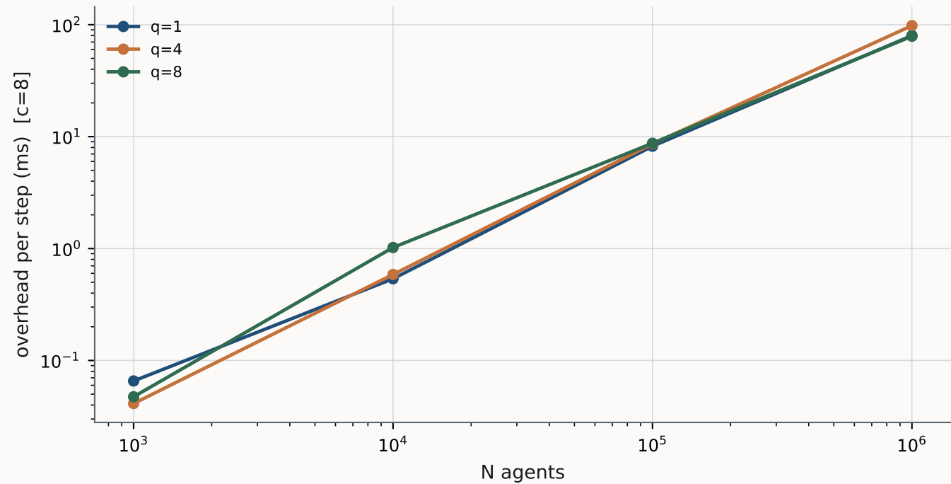
Absolute monitor overhead (check – off) / steps
