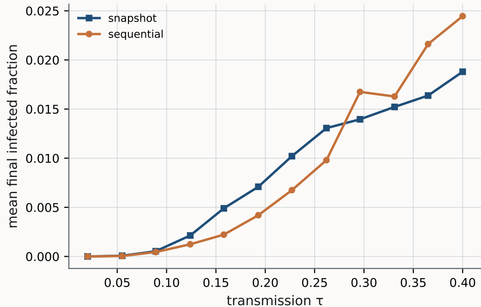
N=2000, steps=80, seeds=48
