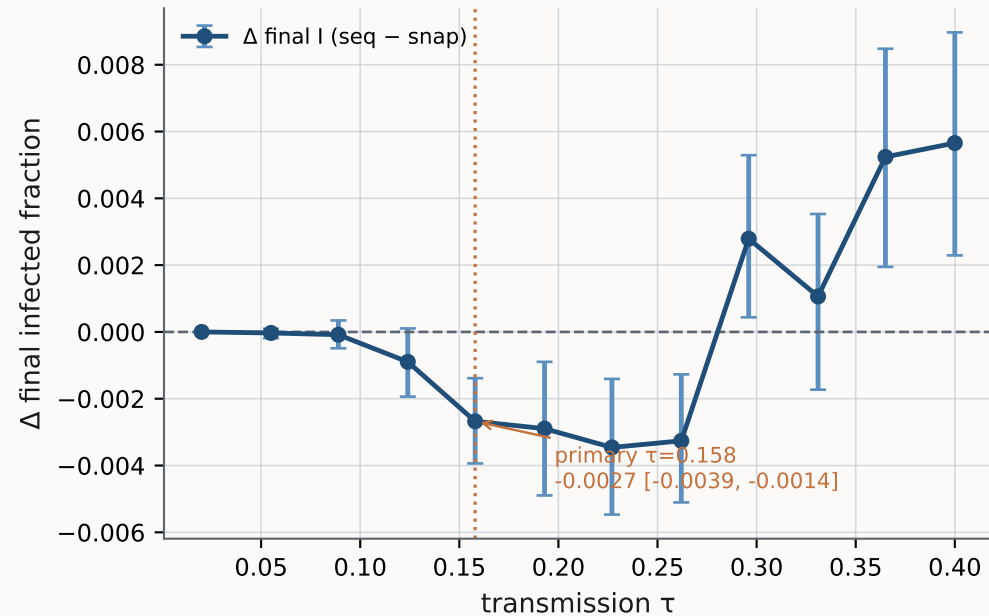
SIR activation effect (shared counter RNG)
